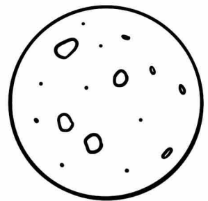
PLUTONE
