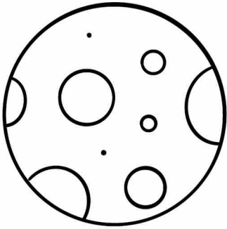
LUNA
