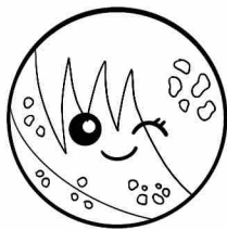
PLUTONE
